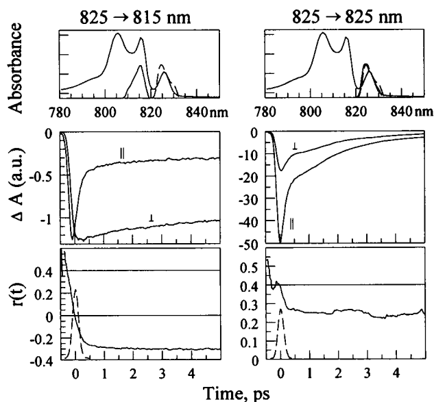
FIGURE 4 Experimental absorption difference profiles (center) and anisotropies (bottom) for FMO trimers from Cb. tepidum excited by 825-nm pulses at 19 K. The experiments are 825 \rightarrow 815 nm (left) and 825 \rightarrow 825 nm (right). Pump and probe pulse spectra (dashed and solid curves, respectively) are superimposed on the steady-state Q_y absorption spectrum in top panels. Dashed curves in the bottom panels are laser auto- or cross-correlations.
